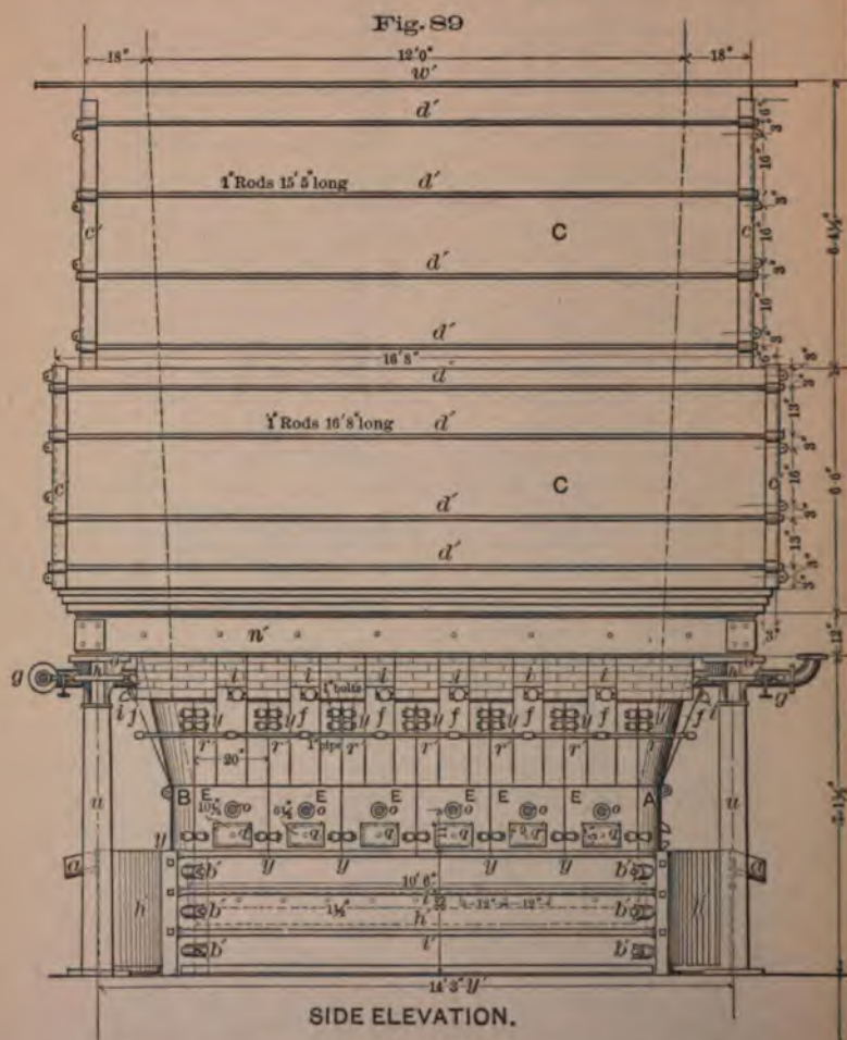
BLAST-FURNACE OF THE GLOBE SMELTING CO.'S WORKS, DENVER, COL.
